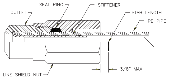
DETAIL "B"
